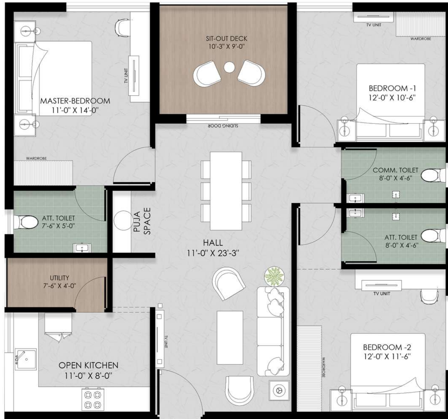
UNIT TYPE -3BHK BUILT UP -1225 SQ .FT
